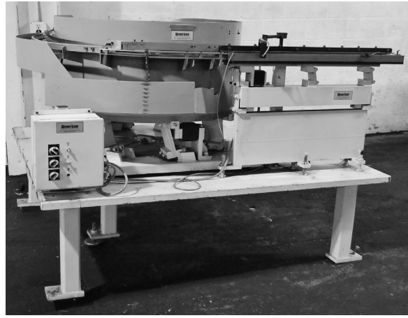
American 48" Vibratory Parts Feeder Bowl/Hopper System
