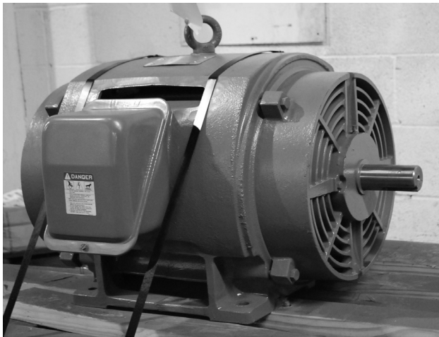
Toshiba 100 HP High Efficiency Motor "New"
