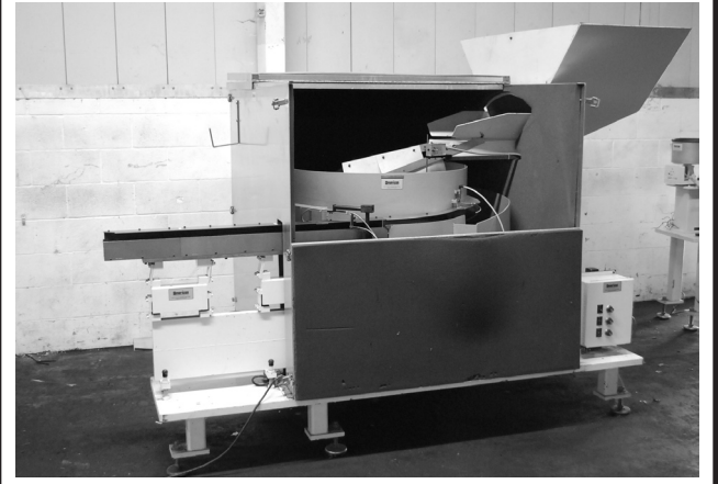
American 48" Vibratory Parts Feeder Bowl/Hopper System
