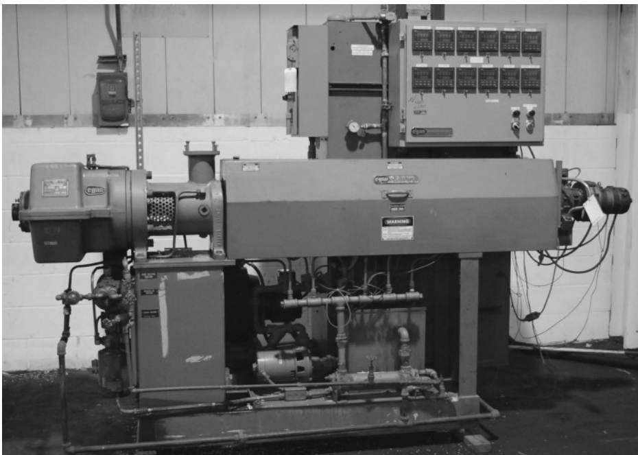
Egan 2 1/2" Plastic Extruder 24:1
