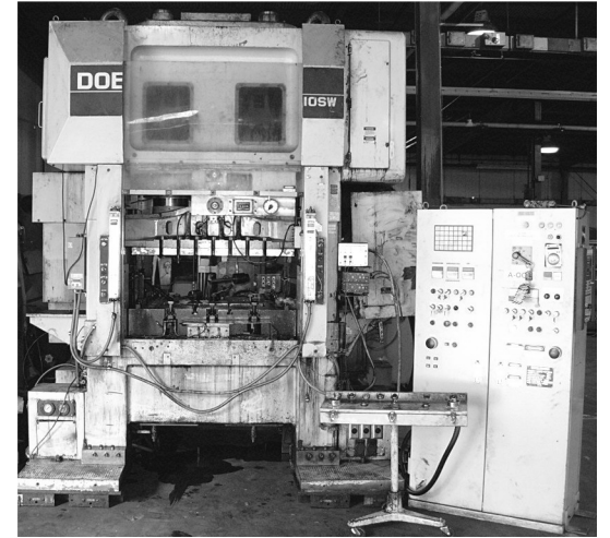
Yamada Dobby #FP-110SW, 110 Ton High Speed Straight Side Press
