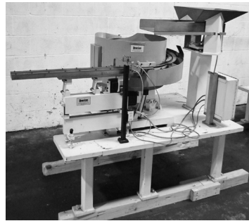
American 36" Vibratory Parts Feeder Bowl
