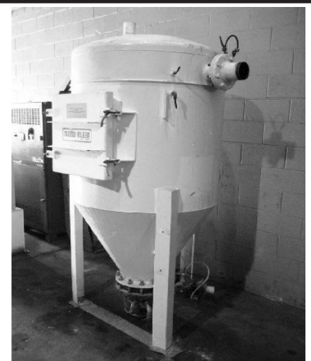
Dynamic Air Dust Filter, 6 Cartridges
