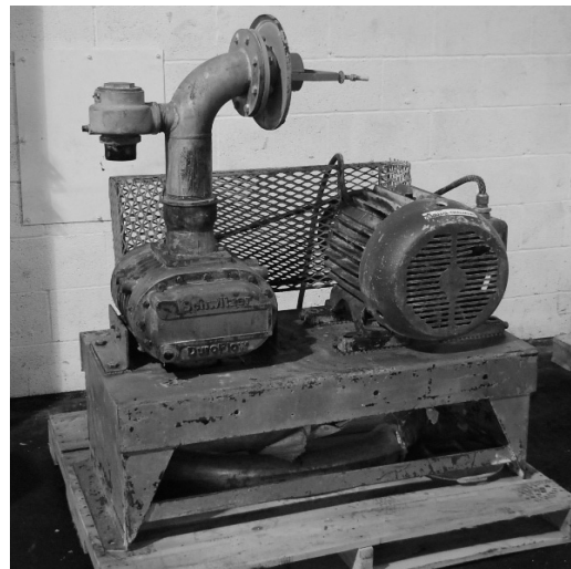
Duroflow Schwitzer #4506, 25HP Rotary Blower
