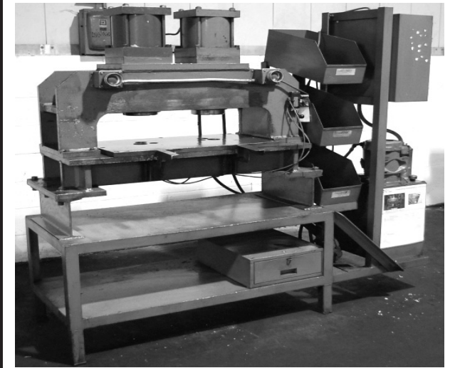
Ortman 12 Ton Dual Cylinder Hydraulic Press
