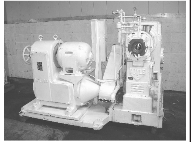
Royle 3" Rubber Extruder
