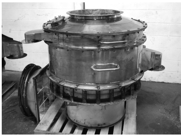
Satos 48" Vibratory Screener, Stainless
