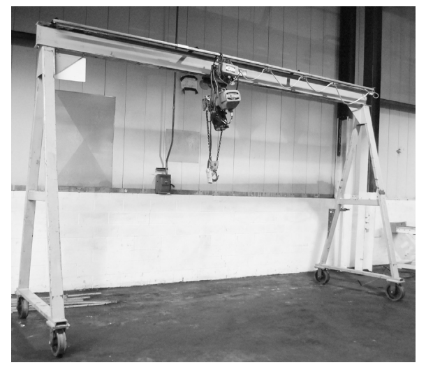
Sacket Systems 4,000# Portable Gantry Crane
