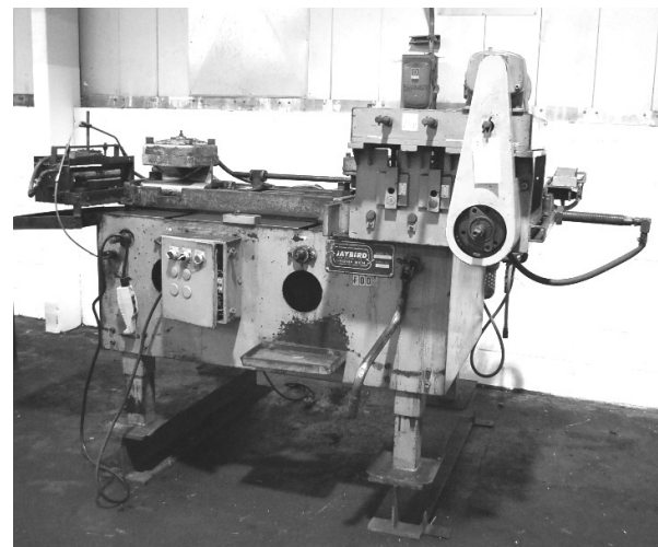
Jaybird #J201818, 18" x .187" Pneumatic Coil Feed/Straightener
