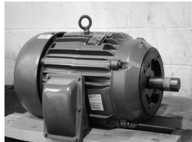
Baldor Super E 20 HP Motor "New"
