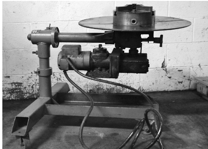
Aronson #AW300, 300# Powered Welding Positioner
