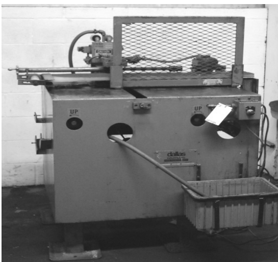
Dallas #D150, 6"x .060 Pneumatic Stock Feeder
